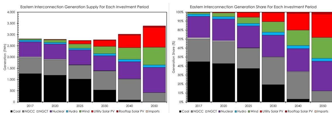
Figure 51: The generation share for the Eastern Interconnection for investment periods. Due to resource scarcity (MW buildout), Wisconsin expands the nuclear capacity across the Eastern Interconnection to provide clean generation in support of the variable generation with storage.
